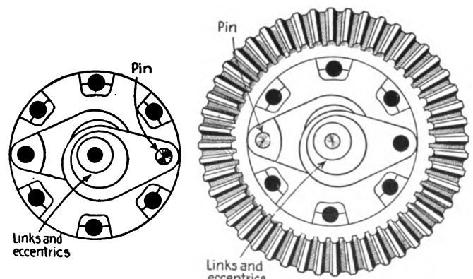
An eccentric can drive a link in and out but cannot be rotated by turning the link around
